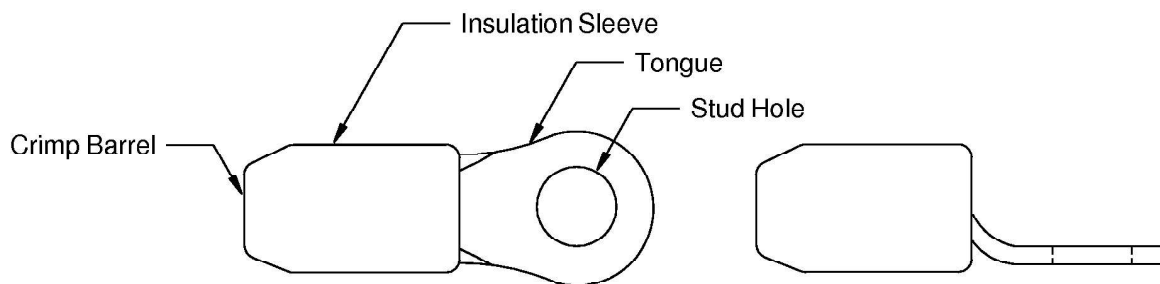
TYPICAL BACT12AL TERMINAL Figure 3
